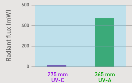
Efficiency of 1W UV-C and 1W UV-A
