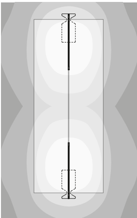
Workplace for six people: Even lighting with two free-standing luminaires
